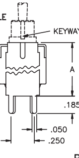
FRONT VIEW DOUBLE POLE
