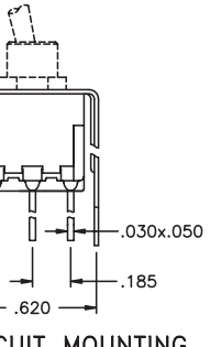
PRINTED CIRCUIT MOUNTING
